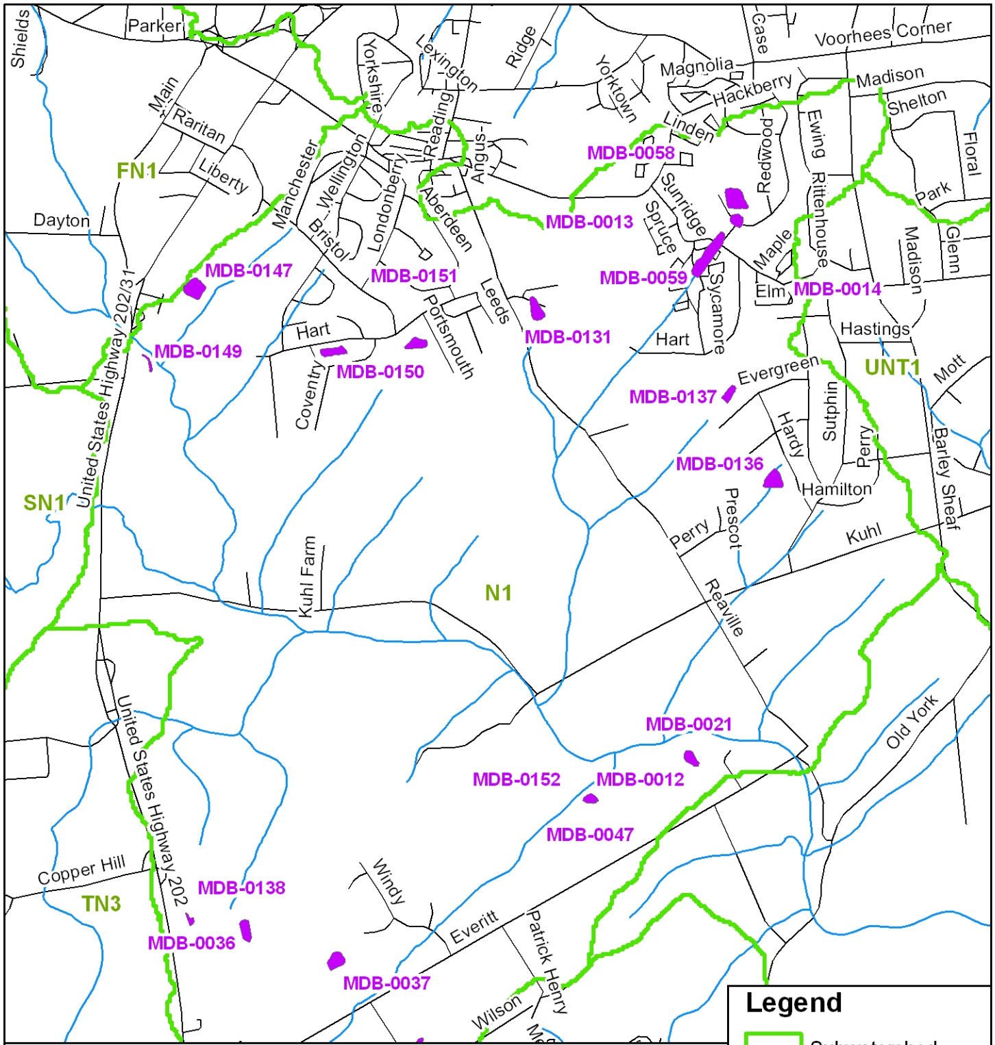
Map of Detention Basins (N1) Neshanic Watershed Restoration Project
